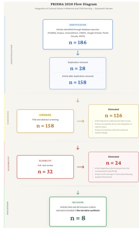
Gambar 1. Diagram PRISMA
